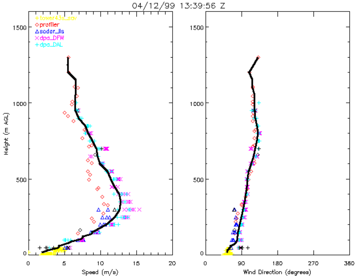
Figure 1. A wind shear case as seen by the AWAS in Dallas. The solid line is the consensus wind profile produced by AWAS, and the sensor measurements are also shown. The AWAS profile shows a wind speed max of about 13 m/s at an altitude of just over 300 m above ground level. The profiler observations, diamonds, show a wind speed maximum of about 10 m/s, while the Dallas Ft. Worth (DFW) and Dallas Love (DAL) TDWR-based Doppler Profile Analysis (DPA) wind profiles show a wind speed maximum of about 14 m/s (three of each DPA are shown, depicting data over the previous 15 minutes).
