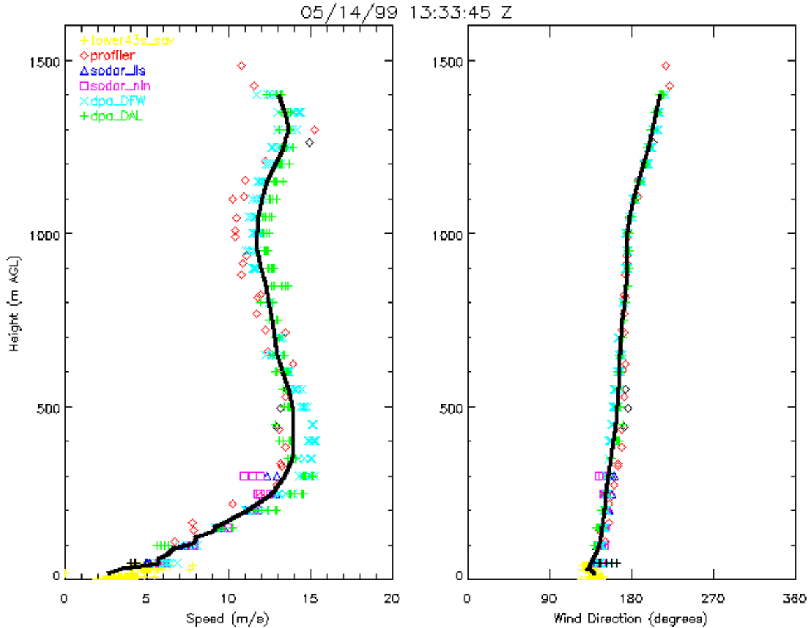
Figure 2. Another wind shear case as seen by the AWAS in Dallas. The solid line is the consensus wind profile produced by AWAS, and the sensor measurements are also shown. In this case the sensors are in very close agreement. The AWAS profile shows a wind speed max of about 14 m/s at an altitude of close to 400 m above ground level. Because the primary runways in DFW are aligned North-South, an aircraft on approach to DFW would experience this wind speed shift as approximately a 23 knot loss of headwind.
