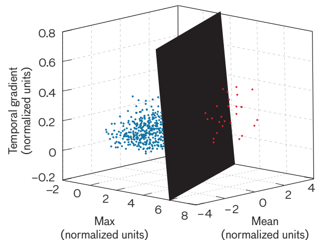
FIGURE 13. This visualization of the feature space used to characterize the sensor network data shows three out of six feature dimensions. A sample set of the field data is plotted, with each point representing the feature values measured within a single time frame. Red points indicate data collected during contaminant release periods of a field test; blue points indicate data collected during background periods. The algorithm learned to use a linear discriminant, shown as the plane in the figure, to separate the contaminant and background data.
