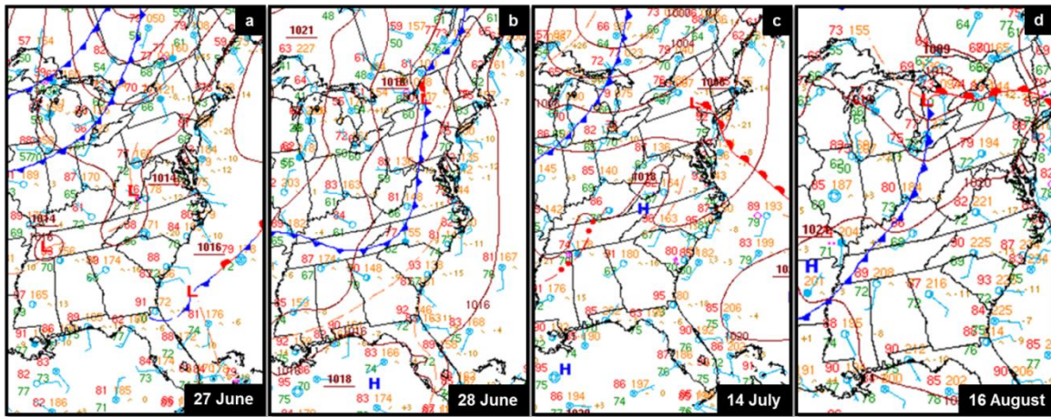
Figure 6. National Weather Service (NWS) 1800 UTC surface pressure and frontal analysis for each observation case day: (a) 27 June, (b) 28 June, (c) 14 July and (d) 16 August 2016.
