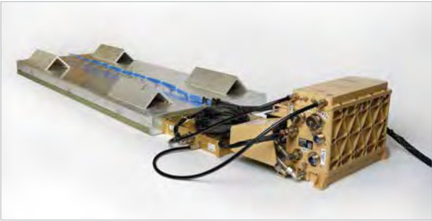
The Localizing Ground-Penetrating Radar system consists of an antenna array (left-hand silver component) and the electronics and processing unit (right-hand section). The system is 1.5 m wide, 7.6 cm tall, and 0.6 m long.
