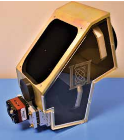
This freeform, optical, very wide field-of-view telescope is ready for testing. The design code of this Lincoln Laboratory-developed optical system optimizes the three mirror surfaces. The mirror surfaces are manufactured with diamond-turning technology and polished to match exactly the design shapes. Assembled and aligned at the Laboratory, the telescope has demonstrated a six-fold improvement in field of view over a design that uses conventional mirrors.
