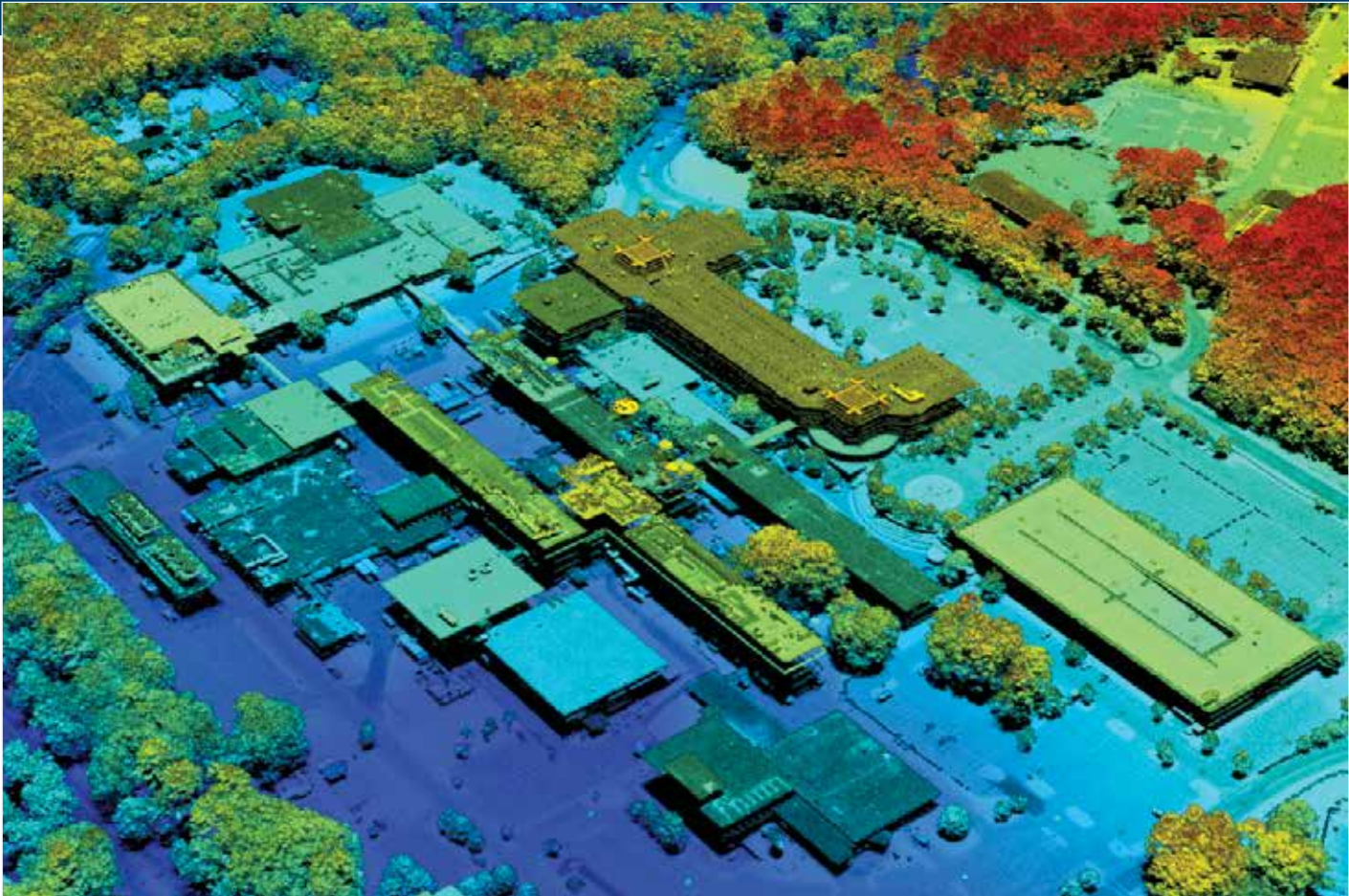
The Multi-look Airborne Collector for Human Encampment and Terrain Extraction, a 3D LADAR designed to uncover clandestine activity in heavily foliated areas, employs photodiode arrays to collect and process data to create 3D images, such as the above image of Lincoln Laboratory.
