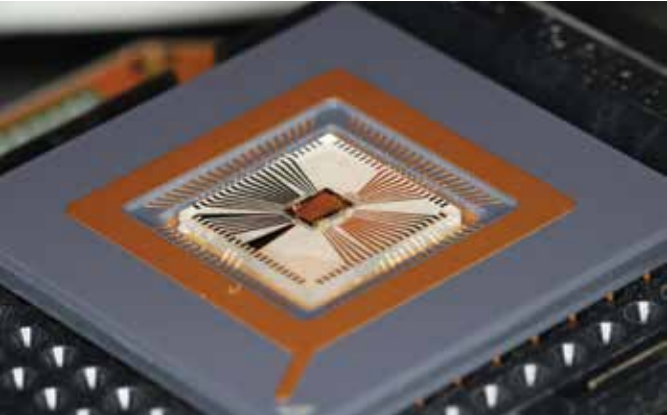
An ion-trap chip is integrated with complementary metal-oxide semiconductor electronics to enable ion movement control in a large-scale quantum processor.
