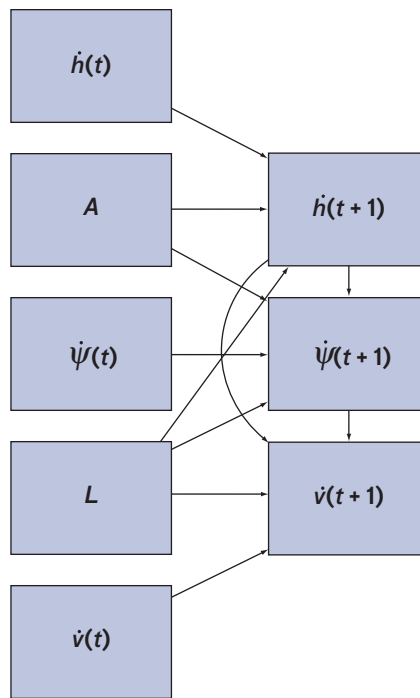
FIGURE 2. This example of a dynamic Bayesian network structure represents the aircraft's state at time t with five variables (vertical rate \dot{h} , airspace class A , turn rate \dot{\psi} , altitude layer L , and airspeed acceleration \dot{v} ), which are linked to three variables describing the state at time t + 1 ( \dot{h} , \dot{\psi} , and \dot{v} ). The arrows show dependencies between variables, represented by using conditional probability tables. For example, the probability of a given turn rate at t + 1 depends on airspace class, altitude, and turn rate at time t , and on vertical rate at time t + 1 .
