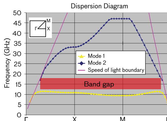
FIGURE 10. Conventional unit cell analysis produces a dispersion diagram showing the propagation modes and the associated band gap. \Gamma , X, and M are the wave vectors, and Mode 1 and Mode 2 are the transverse magnetic and transverse electric low-order eigenmodes.
