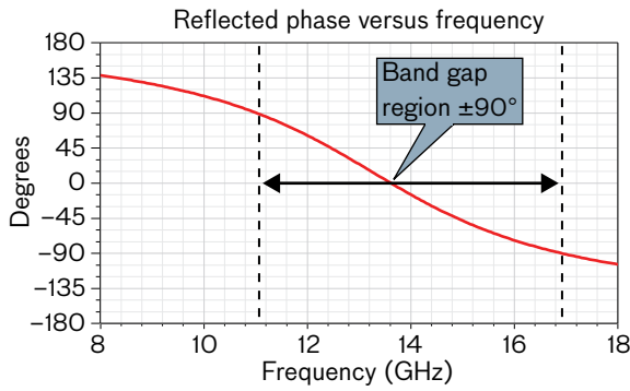
FIGURE 12. The reflected phase off an EBG surface crosses the 0° (perfectly in-phase) reflection point just as the theoretical magnetic conductor would.
