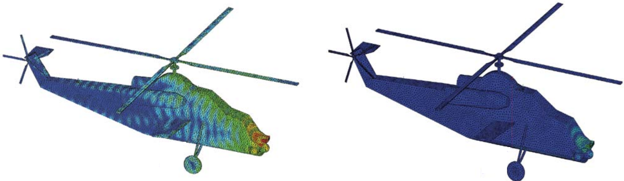
FIGURE 16. The larger test bodies show improvements in both MAGRAM (left) and EBG (right) surfaces, as expected, because of the longer separation between monopoles. Still, the EBG surface is clearly an improvement over MAGRAM and metal (baseline) surfaces.
