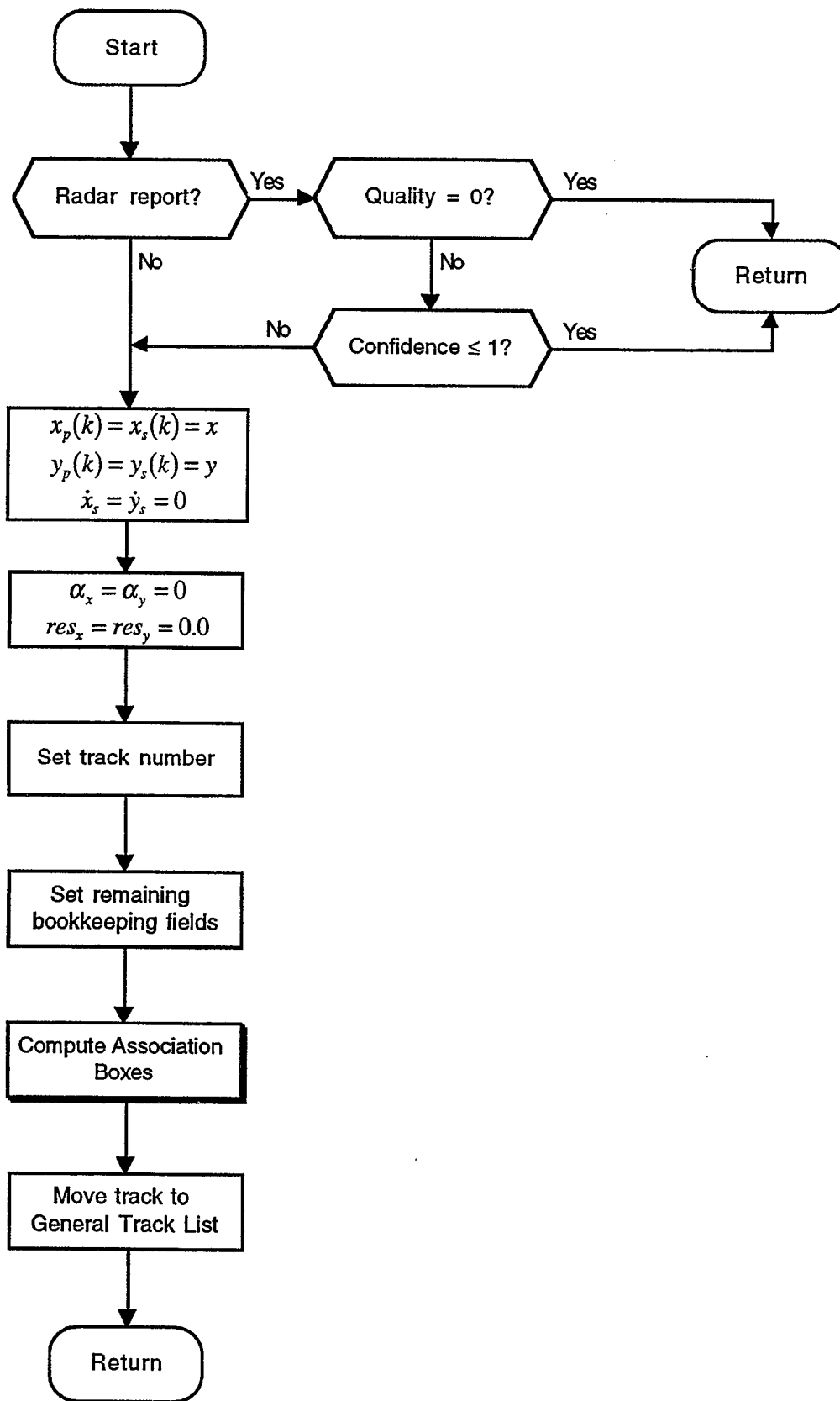
Figure 30. Initiate tracks.
