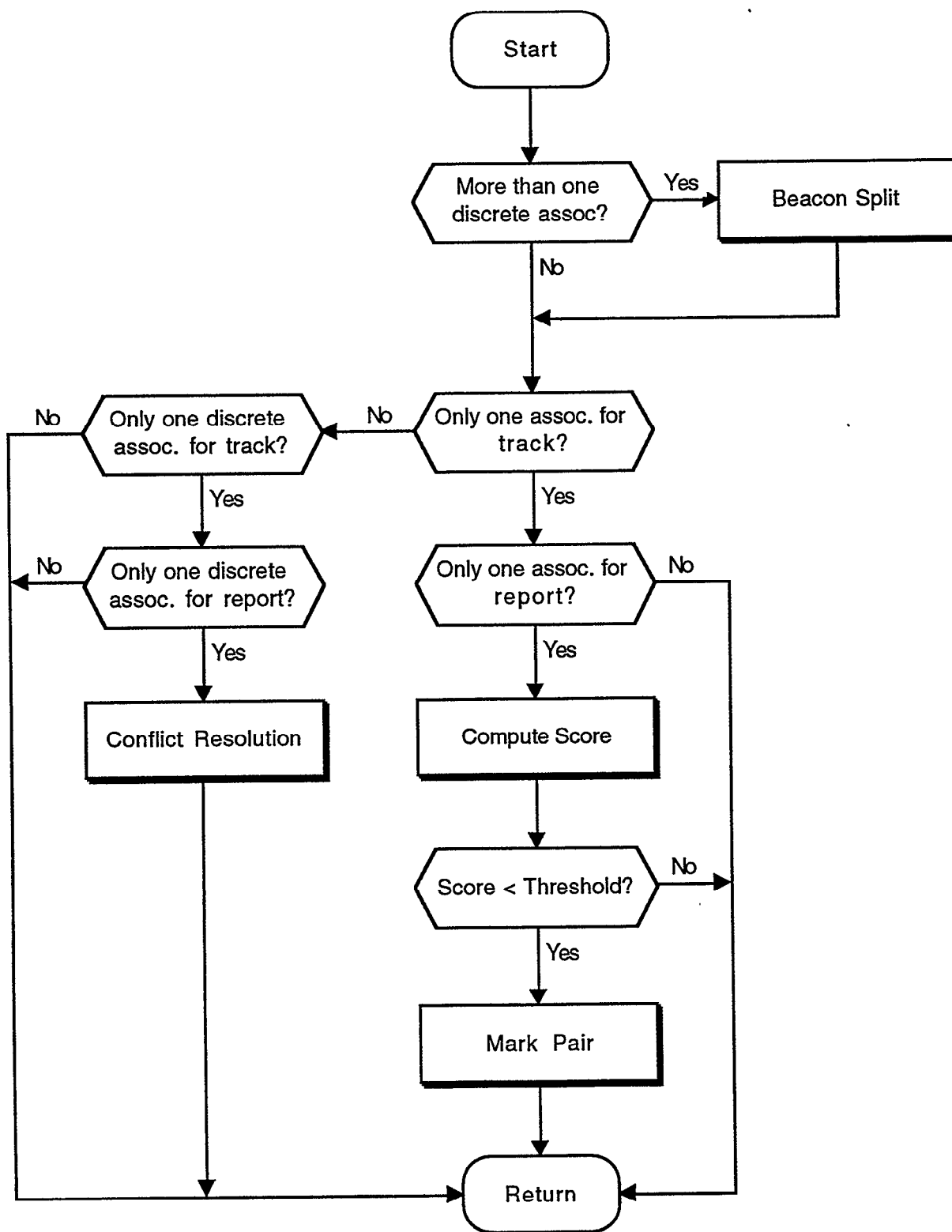
Figure 9. Possibly correlate.
