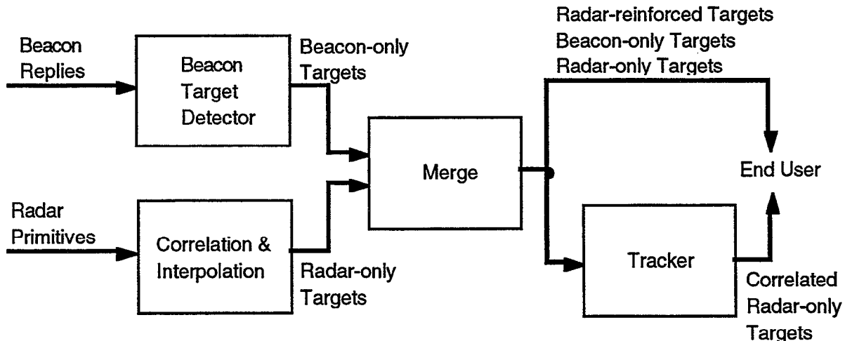
Figure 1. ASR-9 data flow.
