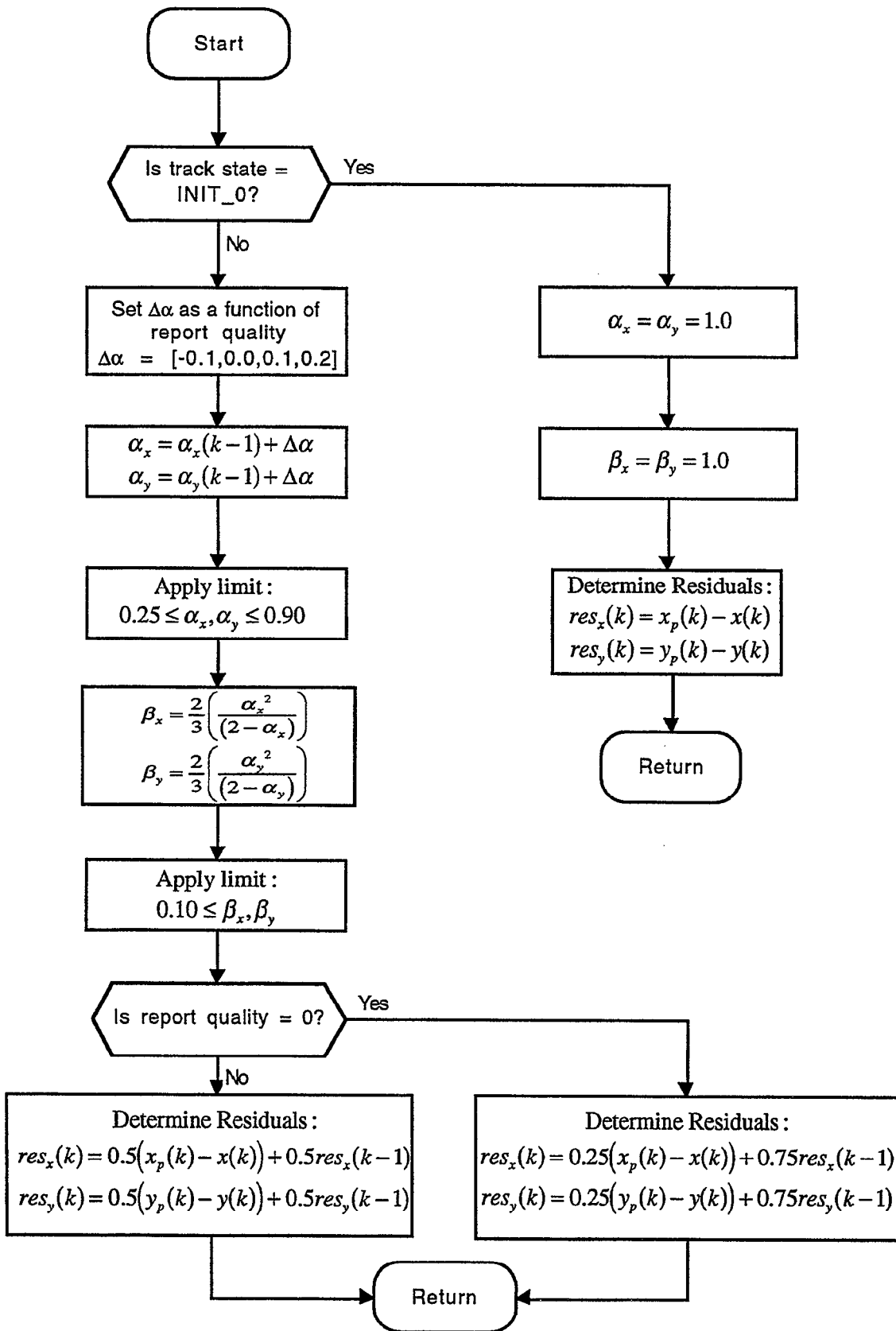
Figure 21. Determine gains.
