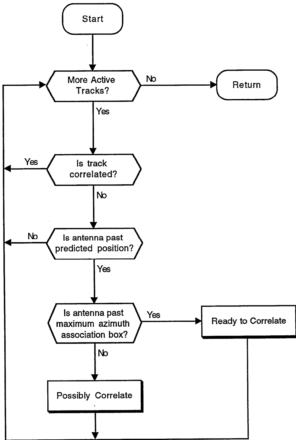
Figure 8. Correlate tracks.
