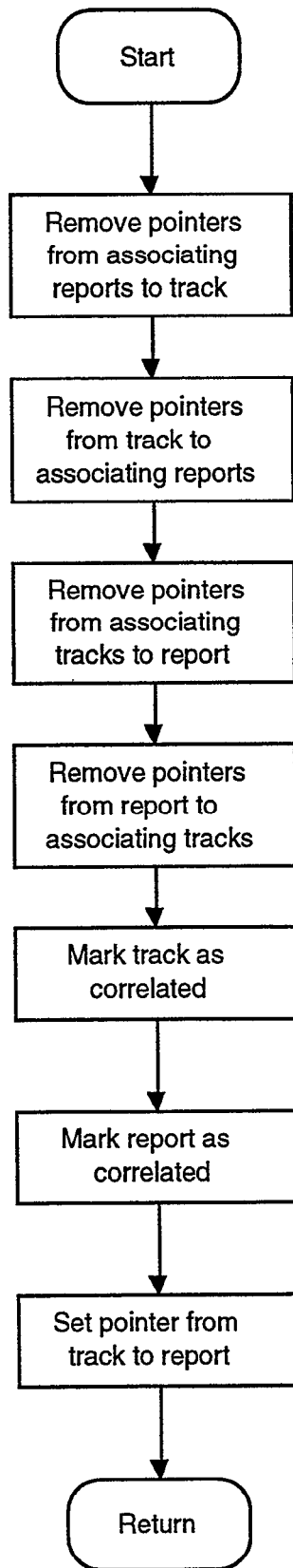
Figure 18. Mark pair.
