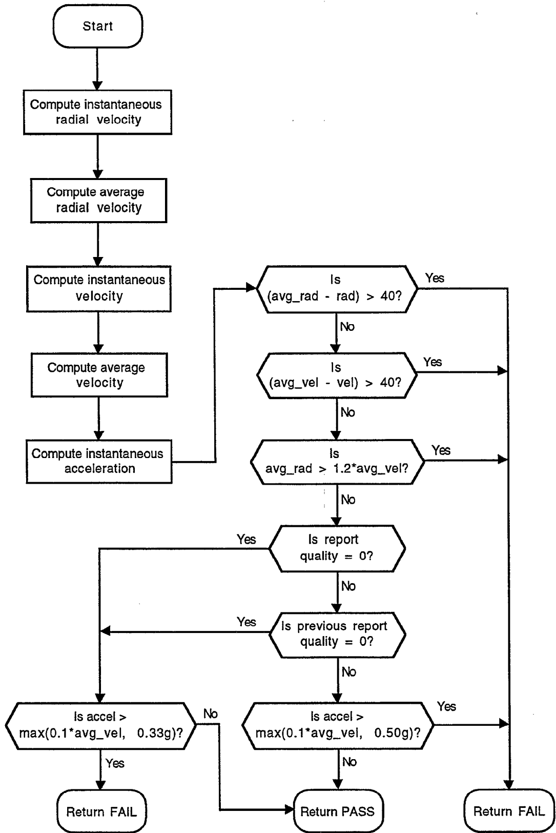
Figure 23. Compute velocity.
