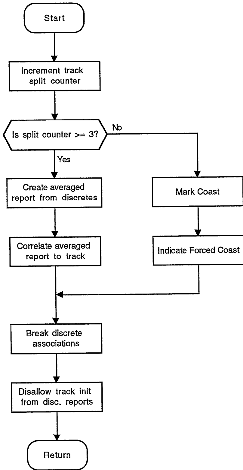
Figure 11. Beacon split.
