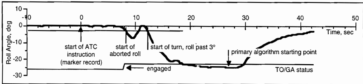
Figure E-2. Roll angle data for a breakout with a double roll. Note return to center after TOGA thrust was engaged.
