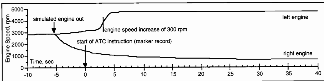
Figure E-4. Engine speed data during a breakout with simulated engine failure.
