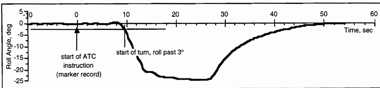
Figure E-1. Roll angle data for a breakout with nominal roll characteristic.
