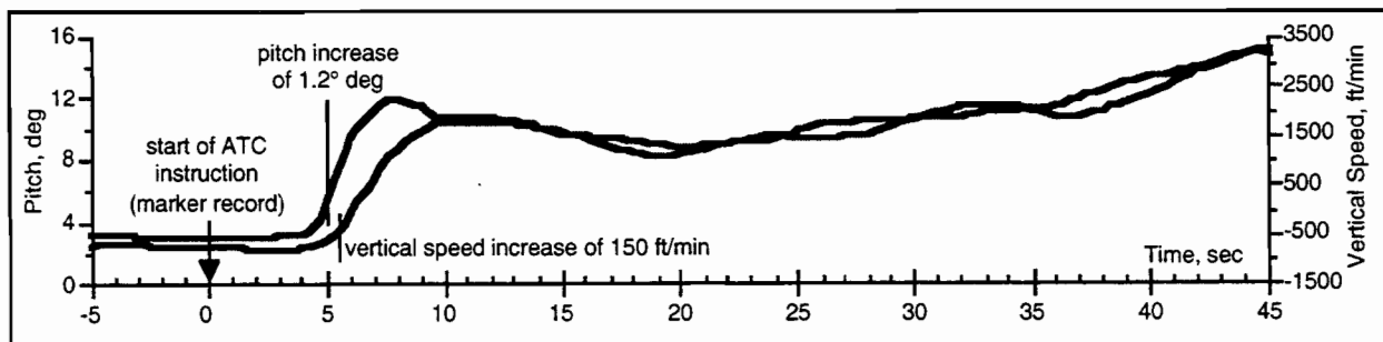
Figure E-3. Pitch and vertical speed data during a breakout.
