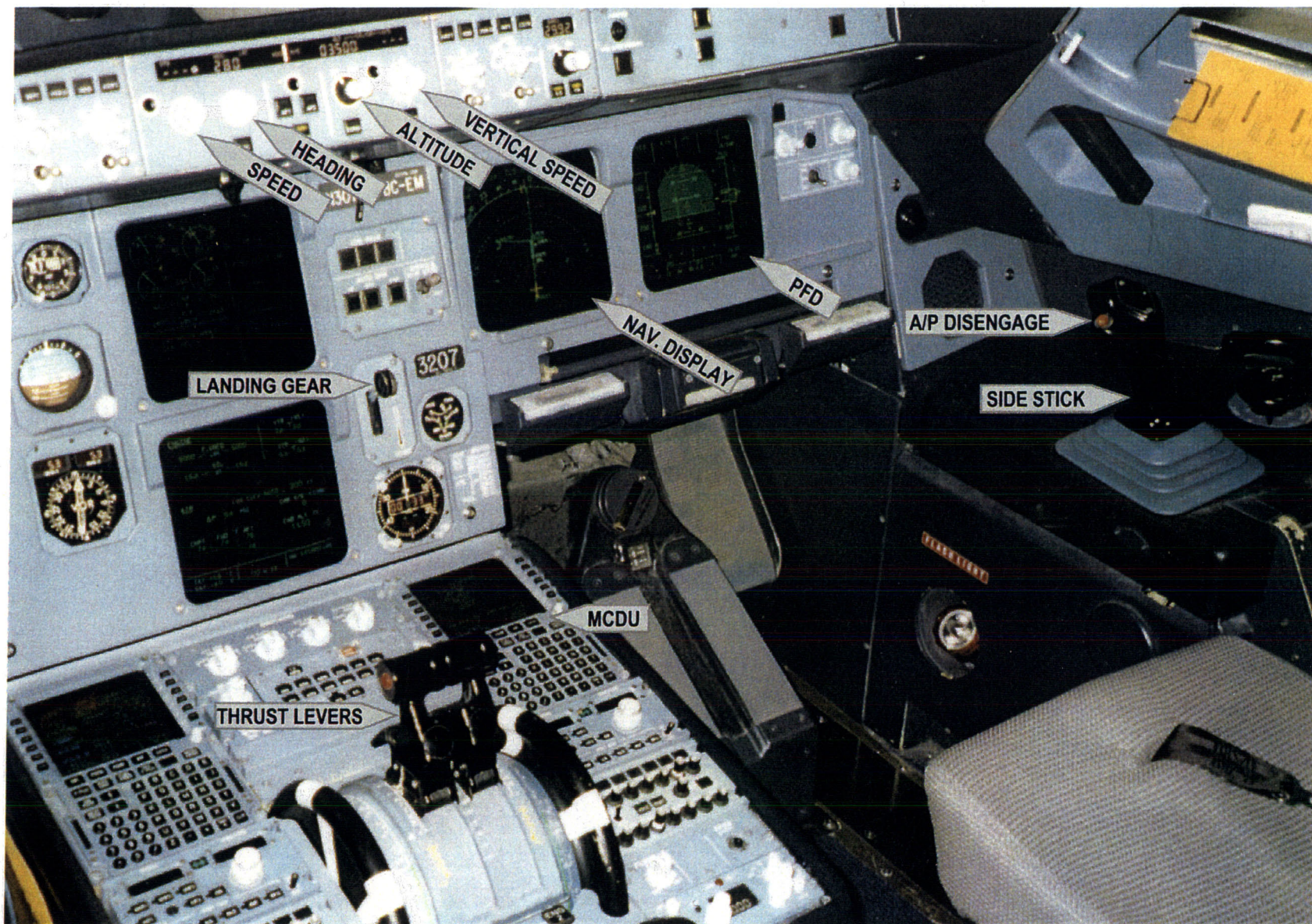
Figure 3-1. A320 flight deck. This view shows the central pedestal and the first officer's side of the instrument panel.
