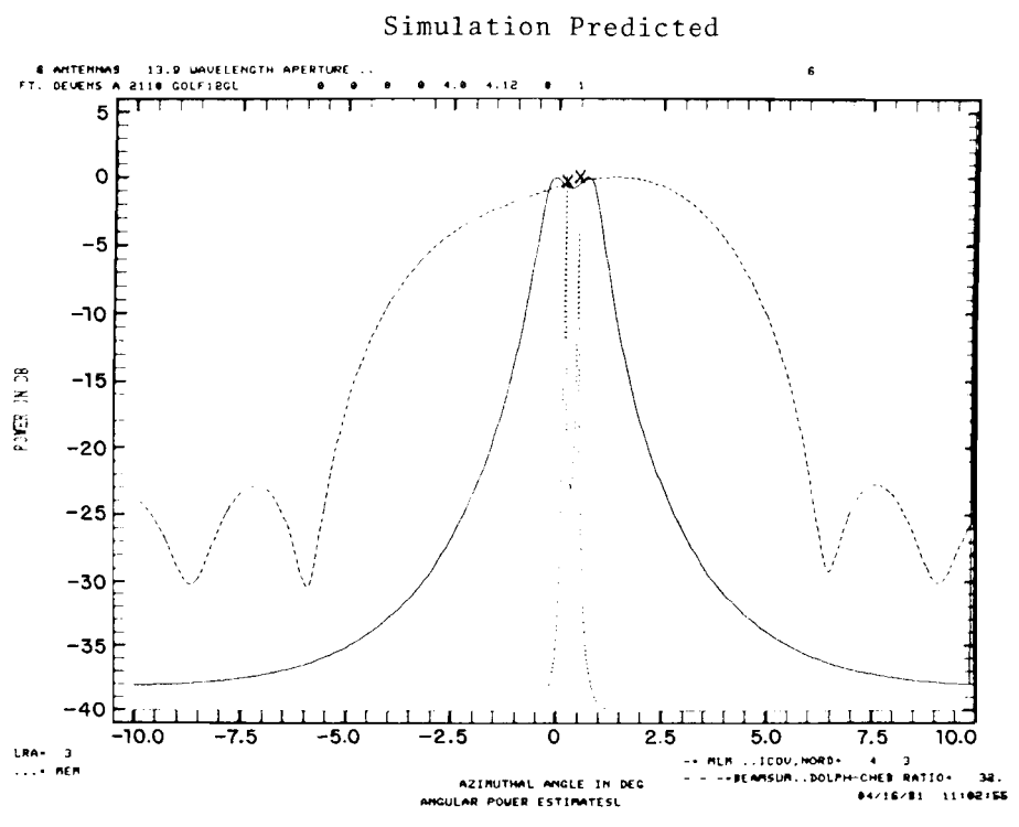
Fig. 5-20. Fort Devens measurement: radial line O-A, L-band azimuth array, \theta_{EL} \approx 4^\circ .
