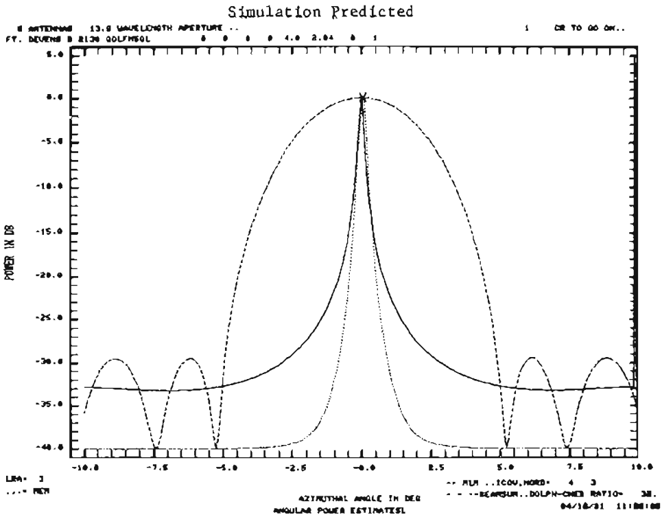
Fig. 5-32. Fort Devens measurement: radial line O-B, L-band azimuth array, \theta_{EL} \approx 2^\circ .
