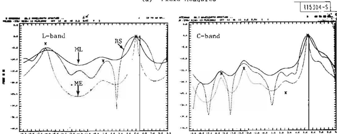
(b) Simulation Predicted (building reflection calculation)
