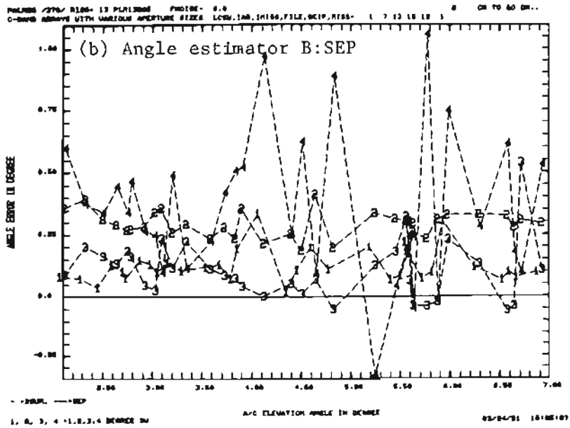
Fig. 6-3. Fort Devens golf course measurement: radial line O-B, angle estimation result.
