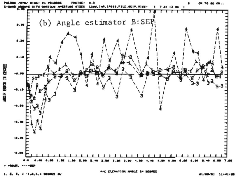
Fig. 6-5. Camp Edwards measurement: Gibbs Road E, angle estimation result.
