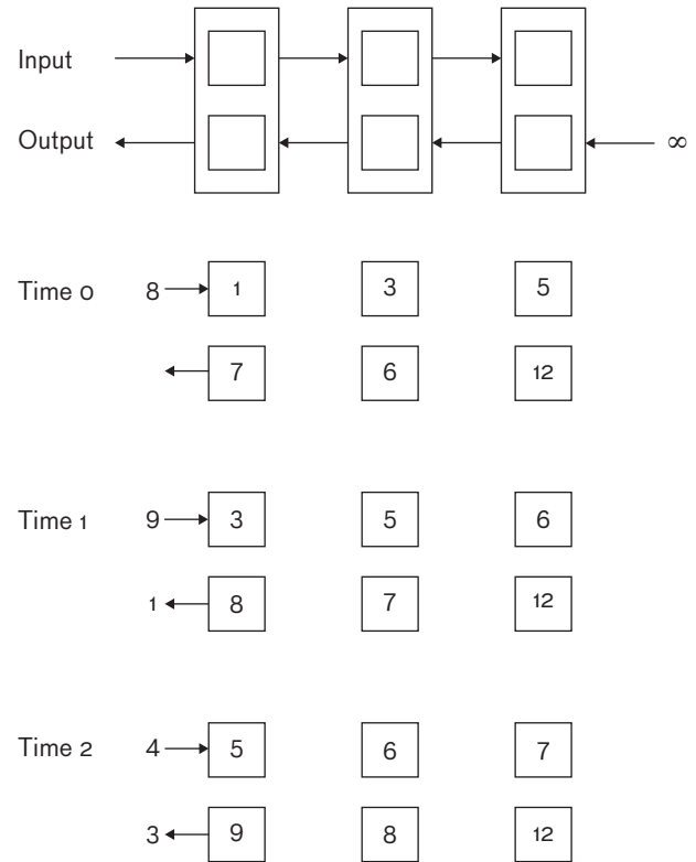
FIGURE 9. The illustration shows the systolic 7-way merge sorter array in operation.
